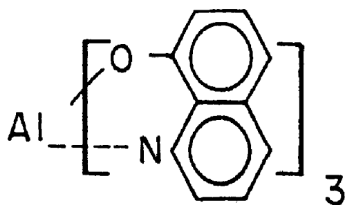
tris(8-hydroxyquinoline) aluminium
