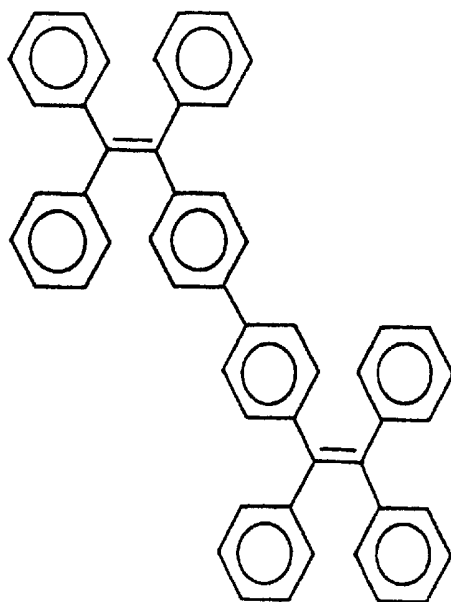
4,4'-bis[(1,2,2-trisphenyl)ethenyl]-biphenyl
